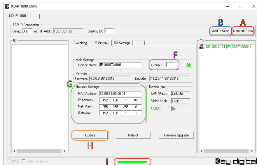
Setup of Tx unit
