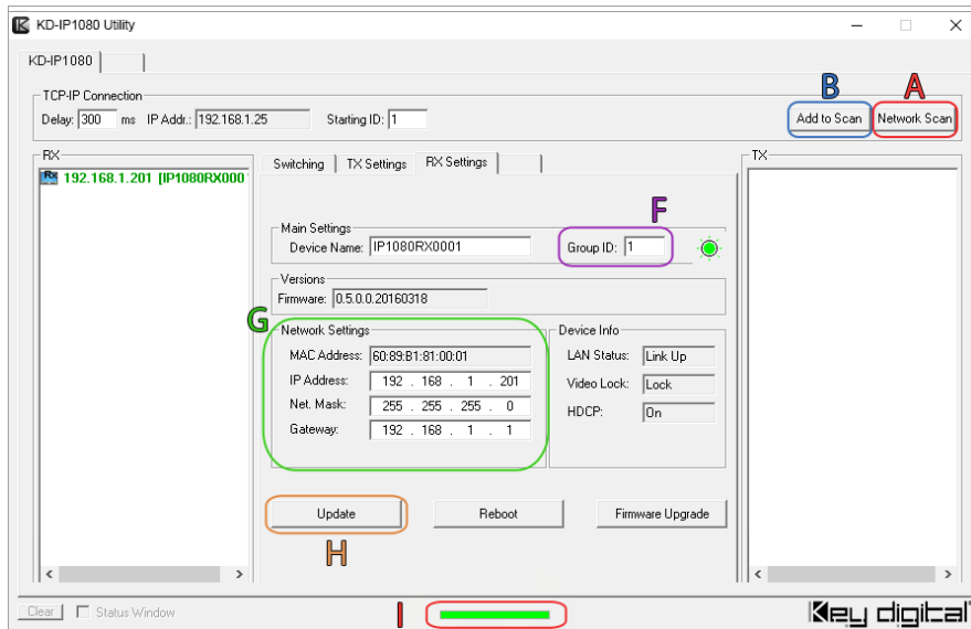
Setup of Rx unit
